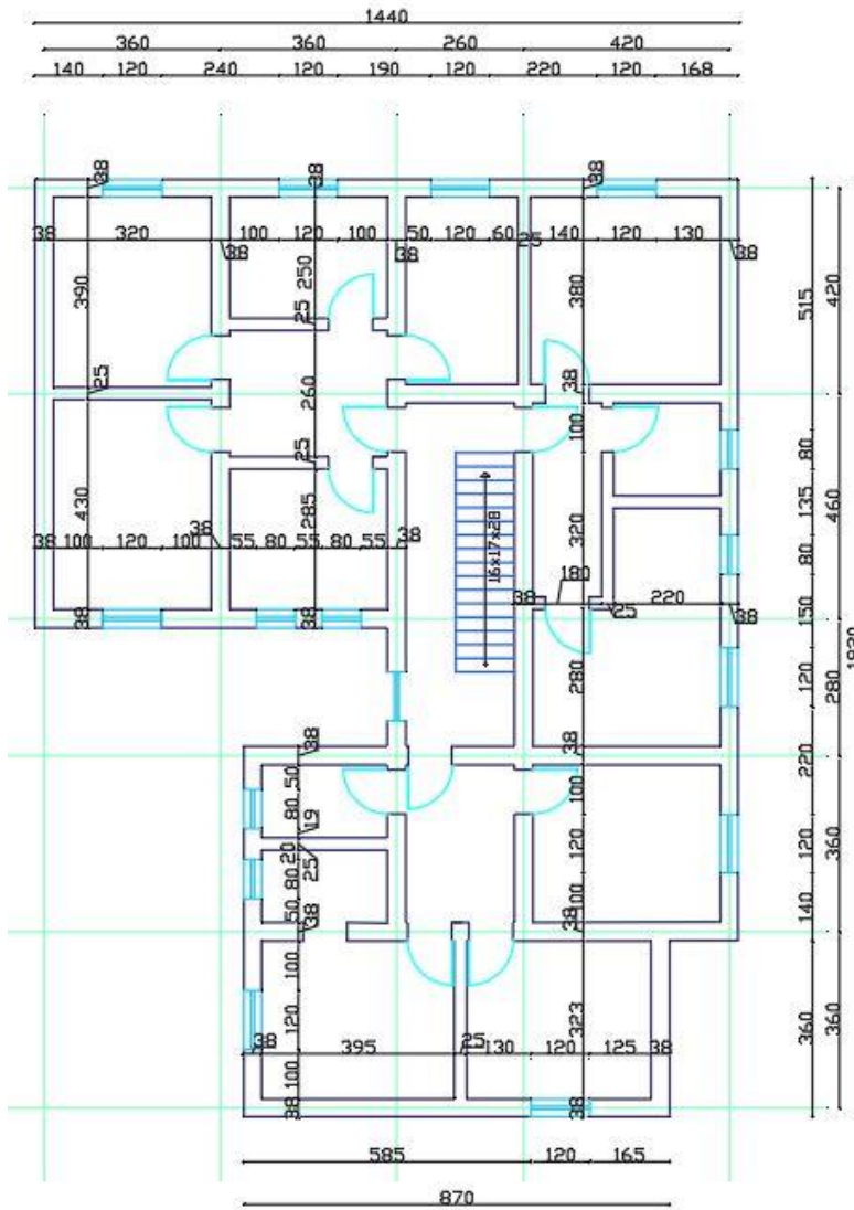
Fig. 1 Typical plan view of the selected masonry building, (units in cm)
