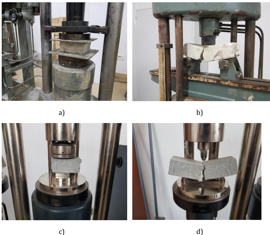
Fig. 2 Brick compression and tensile flexural test (a-b); Mortar samples compression and tensile flexural test (c-d)
