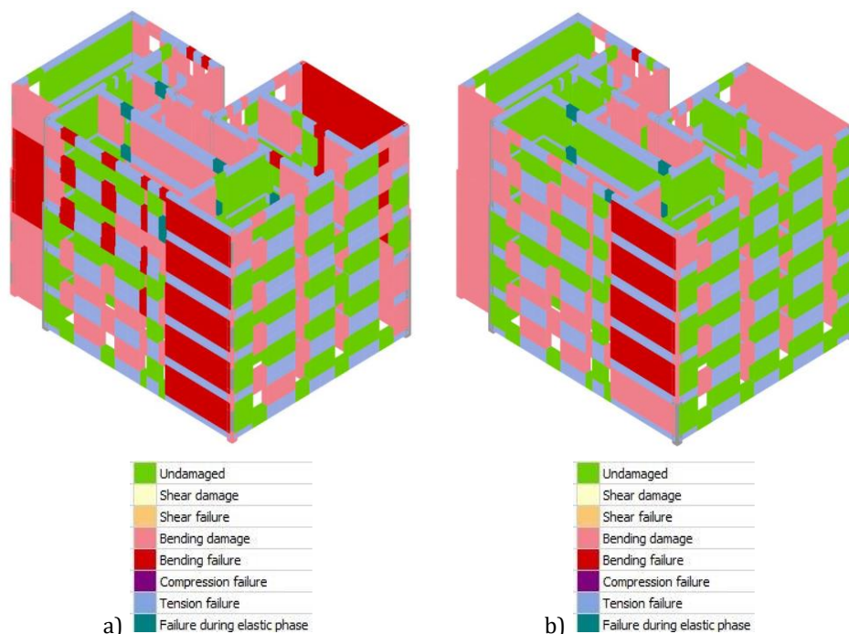
Fig 8. Comparison of the failure mechanism of both buildings; a) Clay brick; b) Silicate brick
